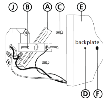
Drawing 2 – Fixture Assembly
