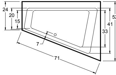
All bathtub dimensions are \pm 1/2 "
